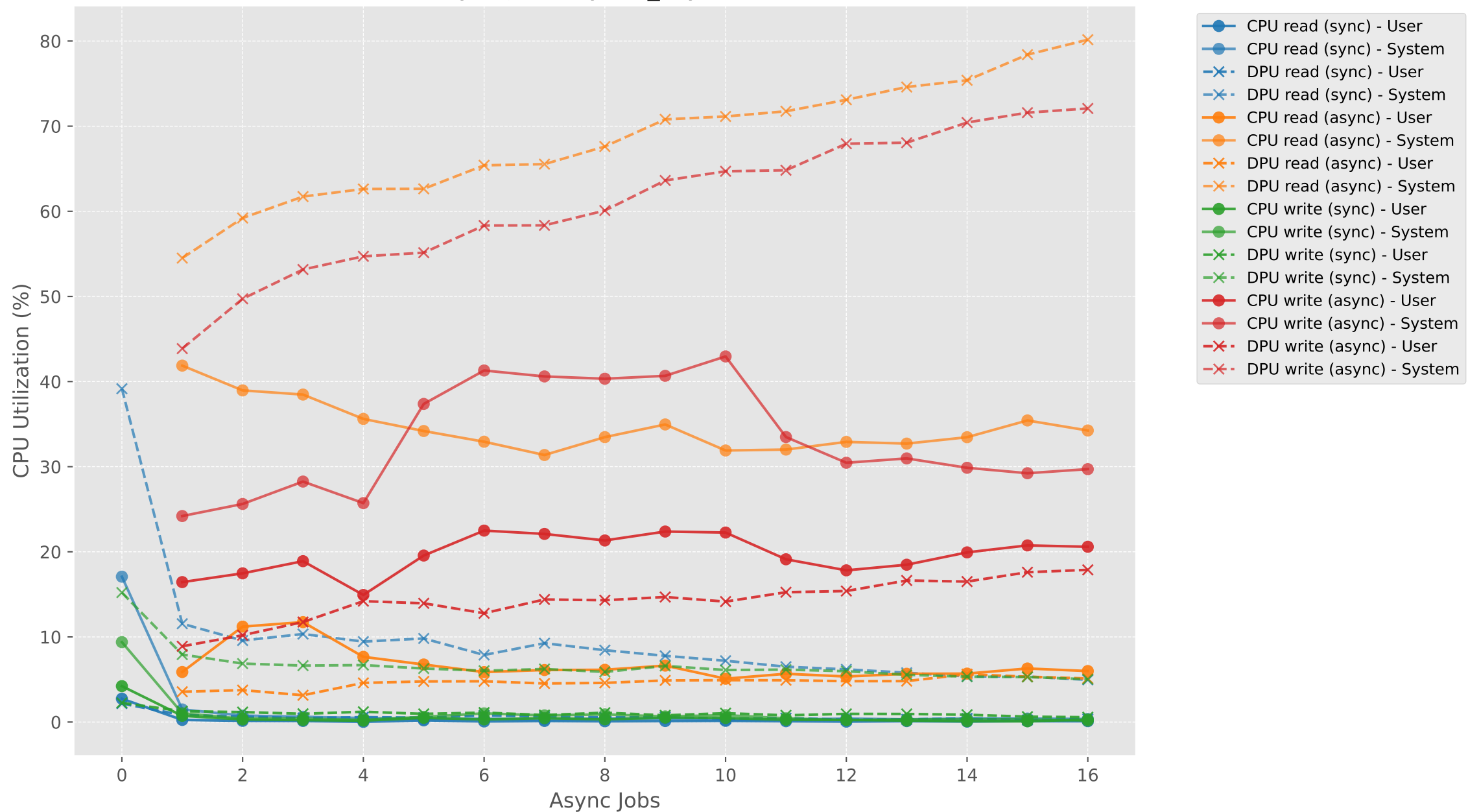
CPU Utilization vs Async Jobs (sync1_asyncN) - SEQ (CPU vs DPU)
